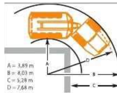
Turning radius according to ISO 7457: 7.68 m
