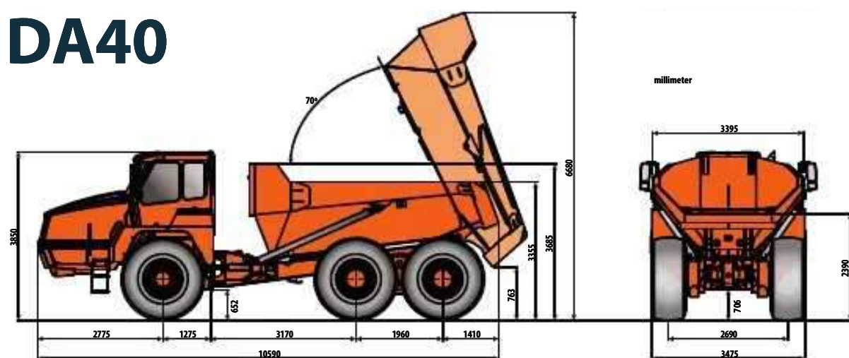
DA40 width with 875/65 R29 tyres: 3630 mm
