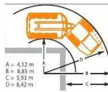
Turning radius according to ISO 7457: 8.42 m
