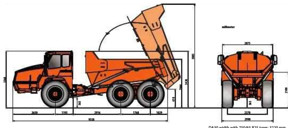
DA30 width with 750/65 R25 tyres: 3220 mm
