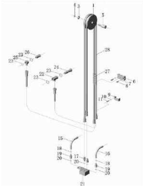
图 109/ Fig.109 第三联附加油路(2 节门架)/3rd hydraulic vavle oil pipe system (Simplex)
