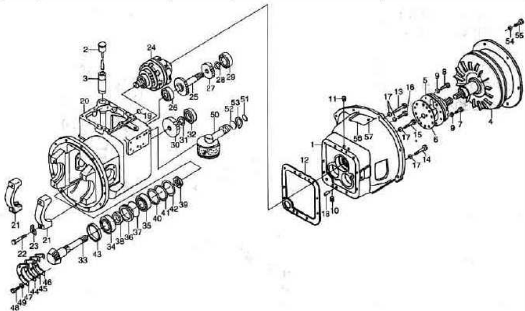
变速箱（液力式）/Gear-box(tor-con type)
