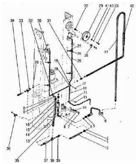
油路系统(3 节门架)/Mast piping (3-Stage mast)
