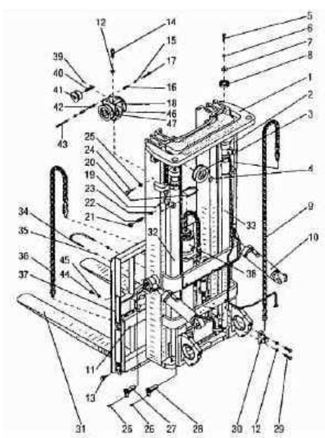
图 121/Fig.121 起升组件(3 节门架)/Lifting part (3-Stage mast)
